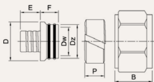
Fordelerkupling eurokonus
